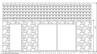
FACHADA PRINCIPAL
